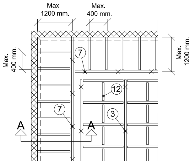
PLAN CUTOUT
