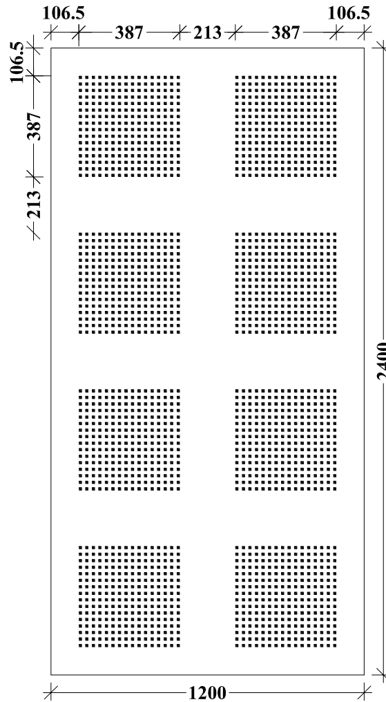
BIG Quattro 46 with the measurement of 1200 x 2400 mm
