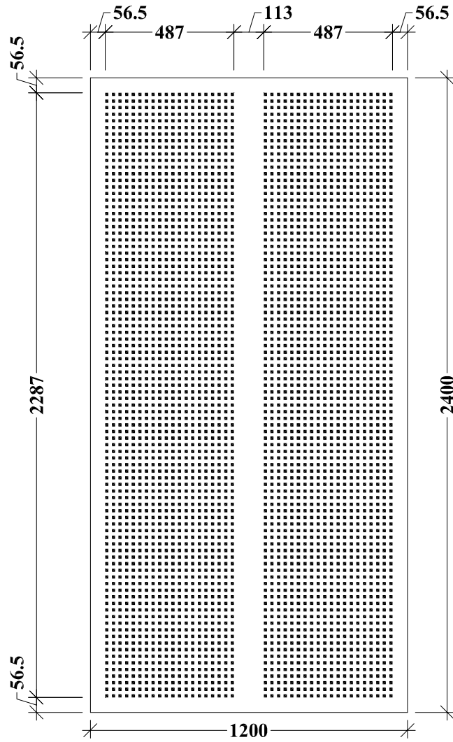
BIG Quattro 41-1 with the measurement of 1200 x 2400 mm
