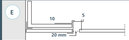
Direct Frieze installed with adjustable bracket and Trap Frieze Profile
