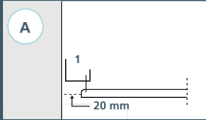
Trap units with: Wall Profile, direct
