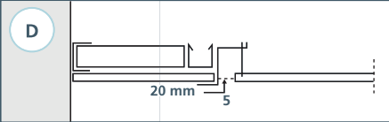
Trap unit with Frieze Profile
