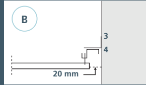
Wall Profile, adjustable
