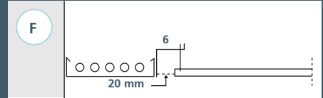
Trap Units mounted against cable tray Profile
